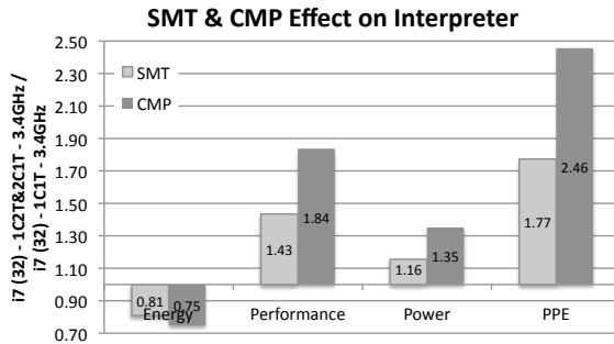
(b) SMT and CMP effect on interpreter.
