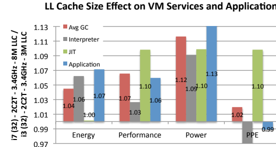
Fig. 6. LL cache size effect on VM services and application
